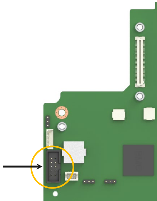
Figure 58. Front panel USB 2.0 connector
