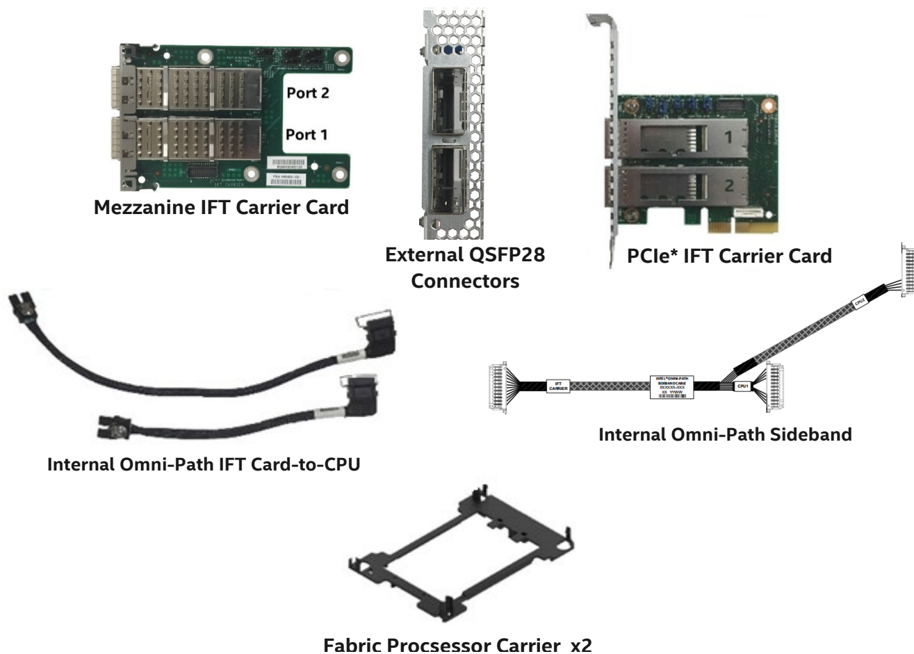
Figure 24. Intel® Omni-Path IFT Carrier Accessory Kit components
