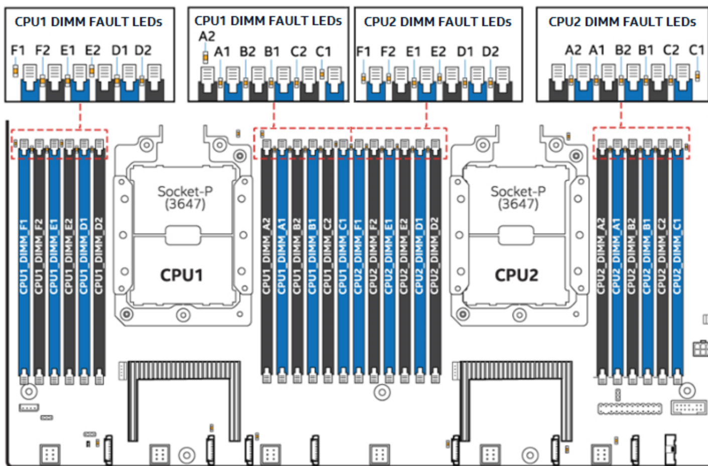
Figure 5. Intel® Light Guided Diagnostics - DIMM fault LEDs
