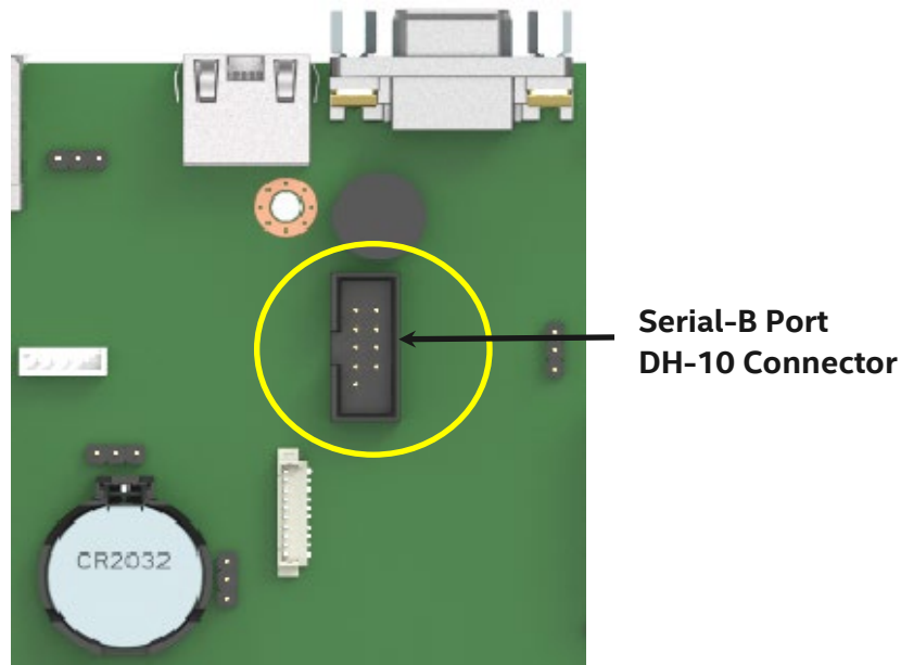
Figure 54. Serial-B connector (internal)
