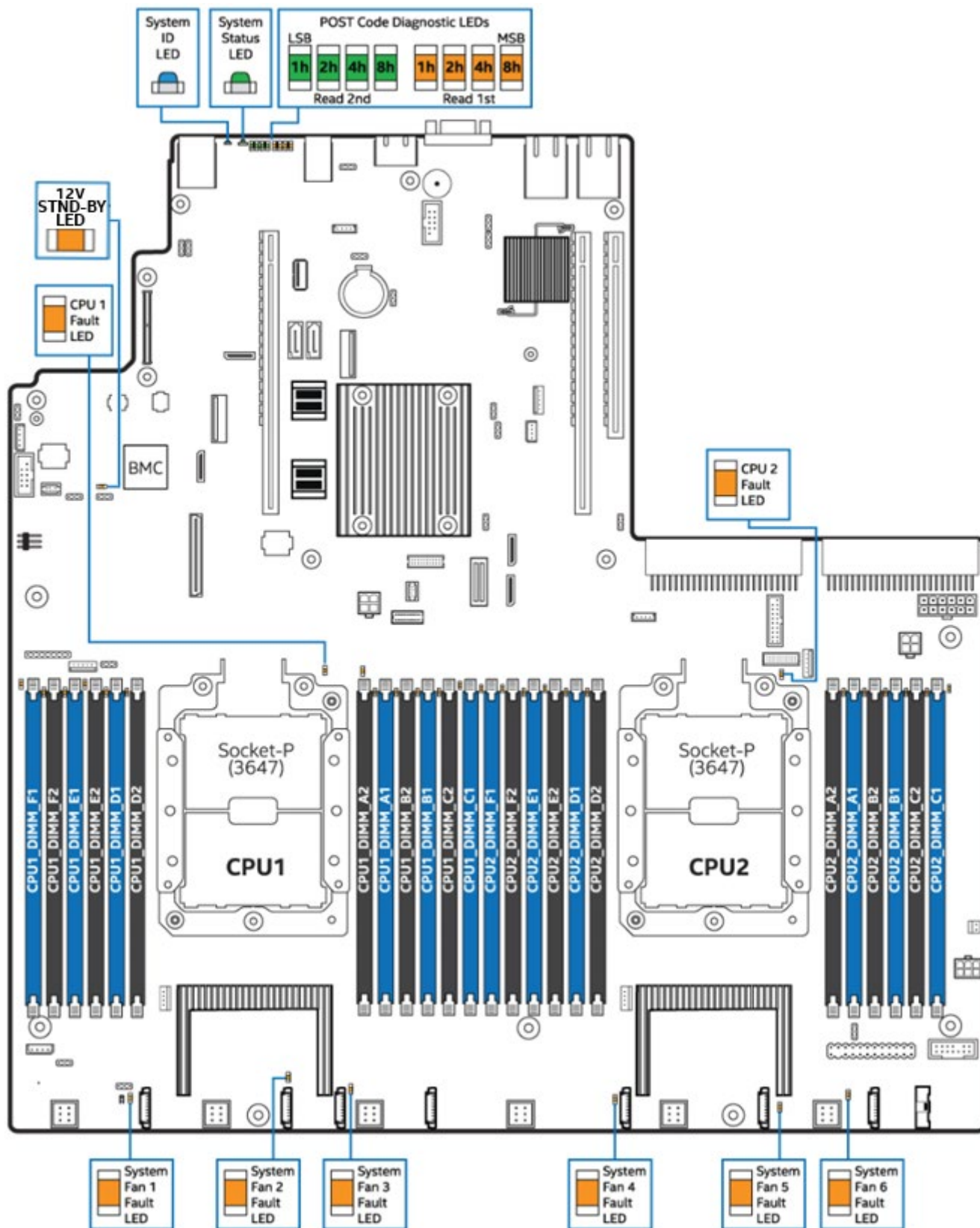
Figure 74. Onboard diagnostic and fault LED placement
