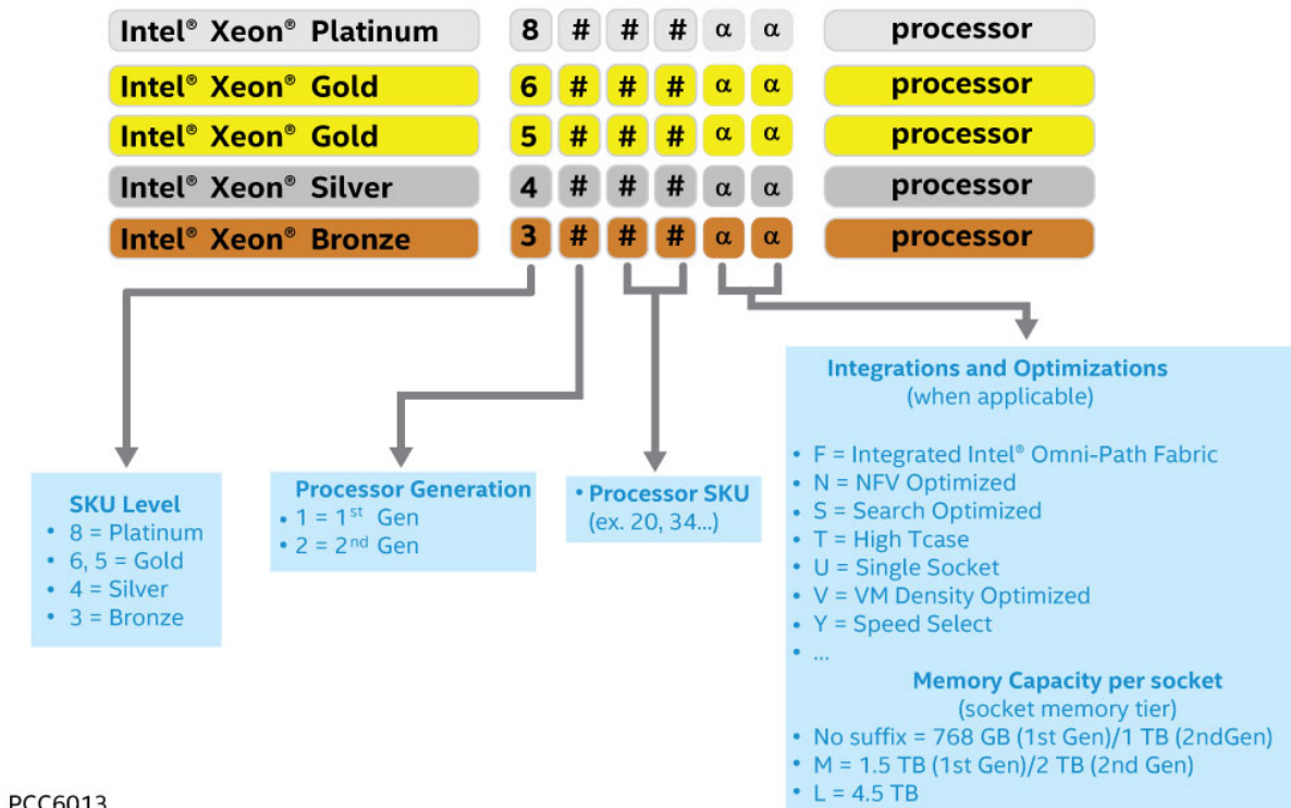
Figure 19. Intel® Xeon® processor Scalable generation identification
