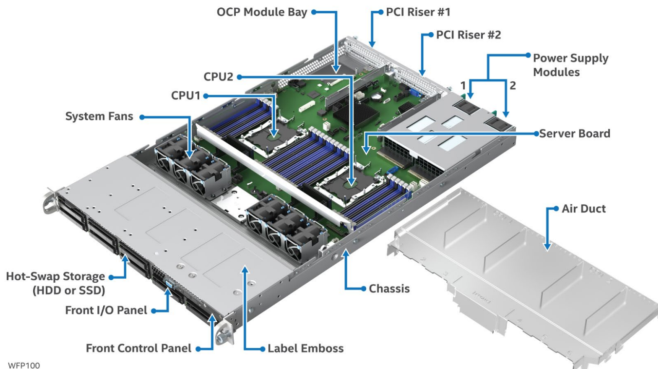
Figure 80. Intel® Server System R1000WF product family
