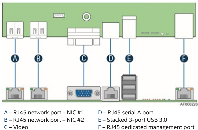
Figure 4. Intel® Server Board S2600WF external I/O connector layout
